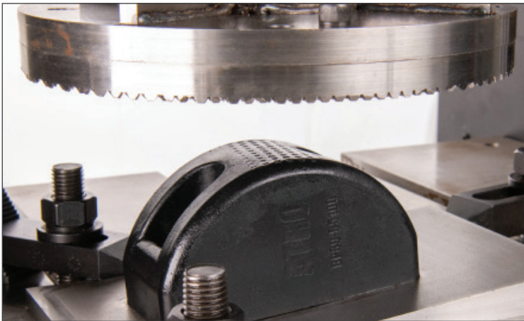
The ATRO polyurethane bumper lasted through 250,000 cycles and was still going strong. The bumper contact surface is still in good shape.
