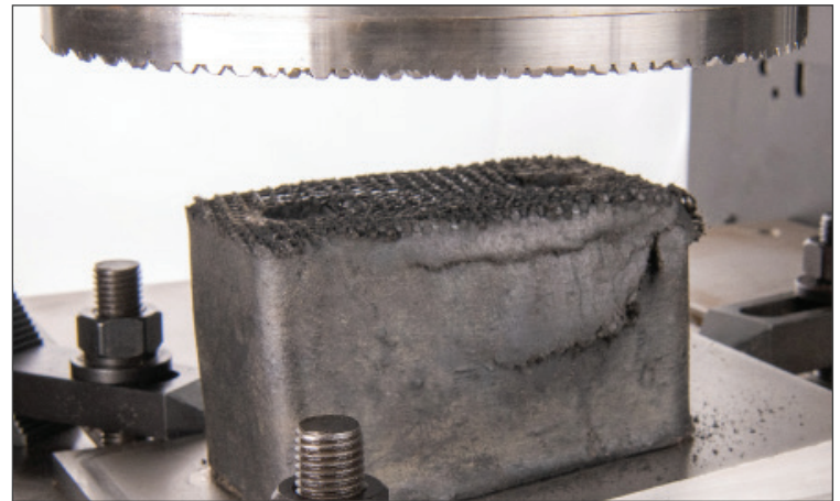
The rubber bumper failed after 16,250 cycles and began to break apart. The bumper contact surface was significantly damaged by the impact.
