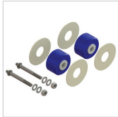
PB50-36322 Pivot Bushing Kit, Narrow, Solid (Shear Bolt) Replaces S-26321 Kit includes shear bolt Shear bolt head snaps off at proper torque
