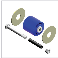
PB50-36914 Pivot Bushing Kit Replaces A-6914 Kit includes hex bolt and bolt sleeve Torque 775-825 ft-lbs
