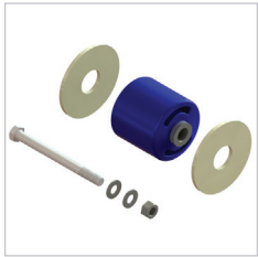
PB50-36000 Pivot Bushing w/Hex Bolt Replaces S-24691 Kit includes hex bolt Torque 500-550 ft-lbs
