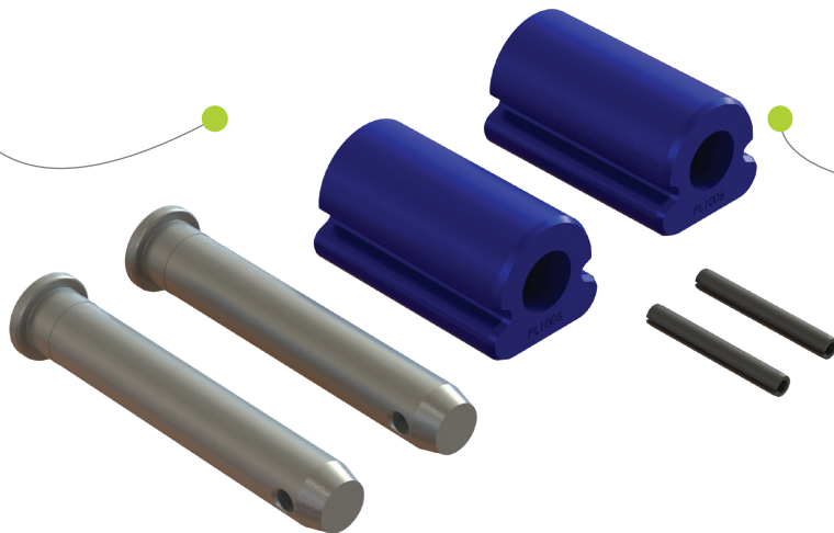
FW51-32413 Foot Pin Repair Kit CAD Rendering
