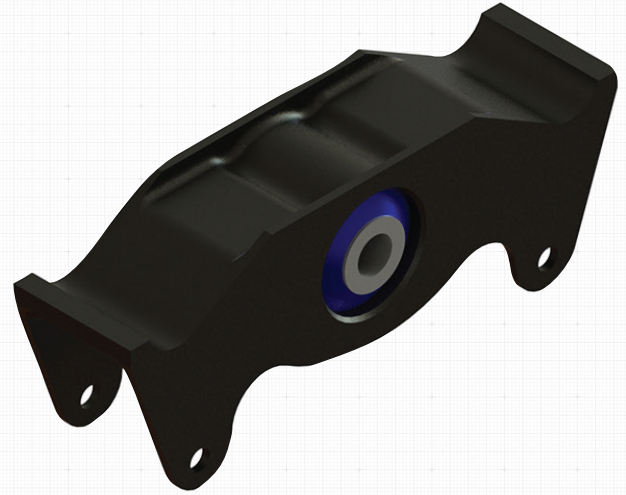
EQ53-35002 Cast Equalizer Beam with Bushing CAD Rendering
