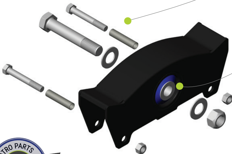
EQ53-35158 Equalizer Beam with Bushing (Kit) CAD Rendering
