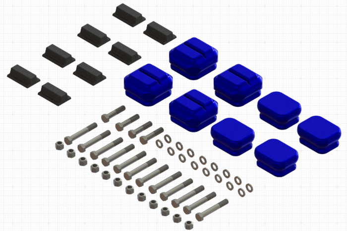
SK62-50380 Insulator Kit w/Hdwr & Spacer Blocks (CAD Rendering)
