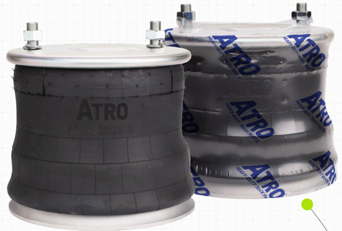
AS1R-8050-A Rolling Lobe with Aluminum Piston Showing shrink-wrapped packaging
